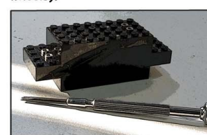
Put the motor in the gear and check the right position of the brass gearwheel.
